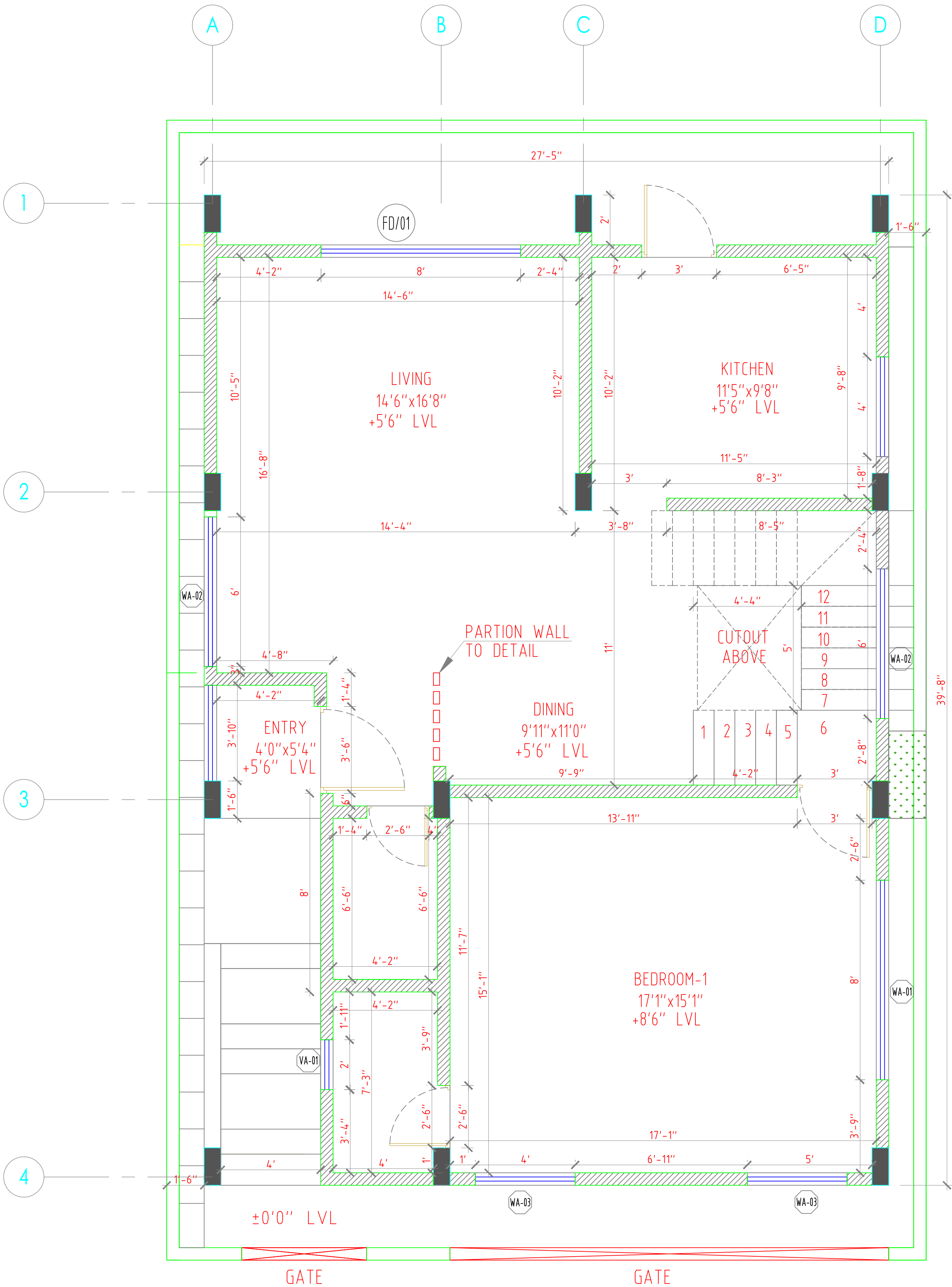
GROUND FLOOR PLAN - LEVEL 1 01
